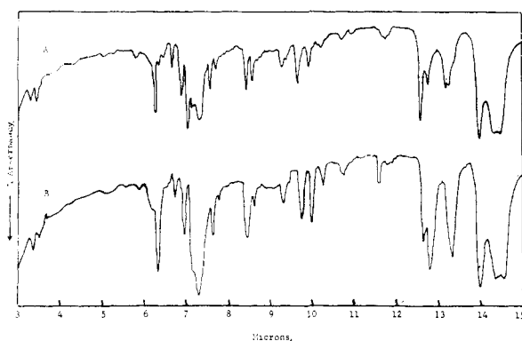
Fig. 1.—Infrared spectra of 1,2,3,4-tetraphenylcyclobutadienepalladium(II) chloride (A) and of 1,2,3,4-tetraphenylcyclobutadienenickel(II) bromide (B) in potassium bromide disks.
